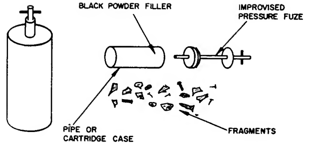
Figure 18. VC "toe popper" mine.
